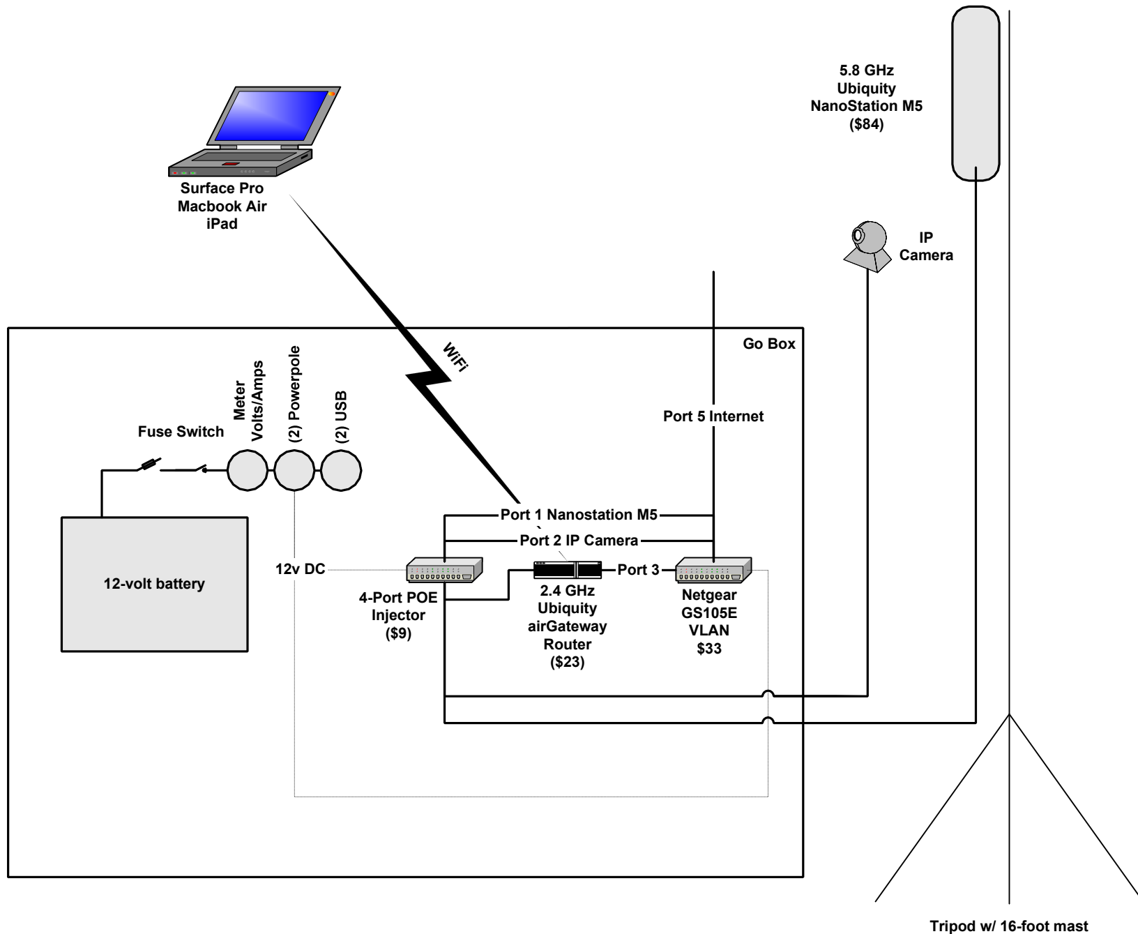
AL7MH Portable AREDN Mesh Network Station
